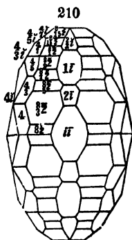
Humite.
